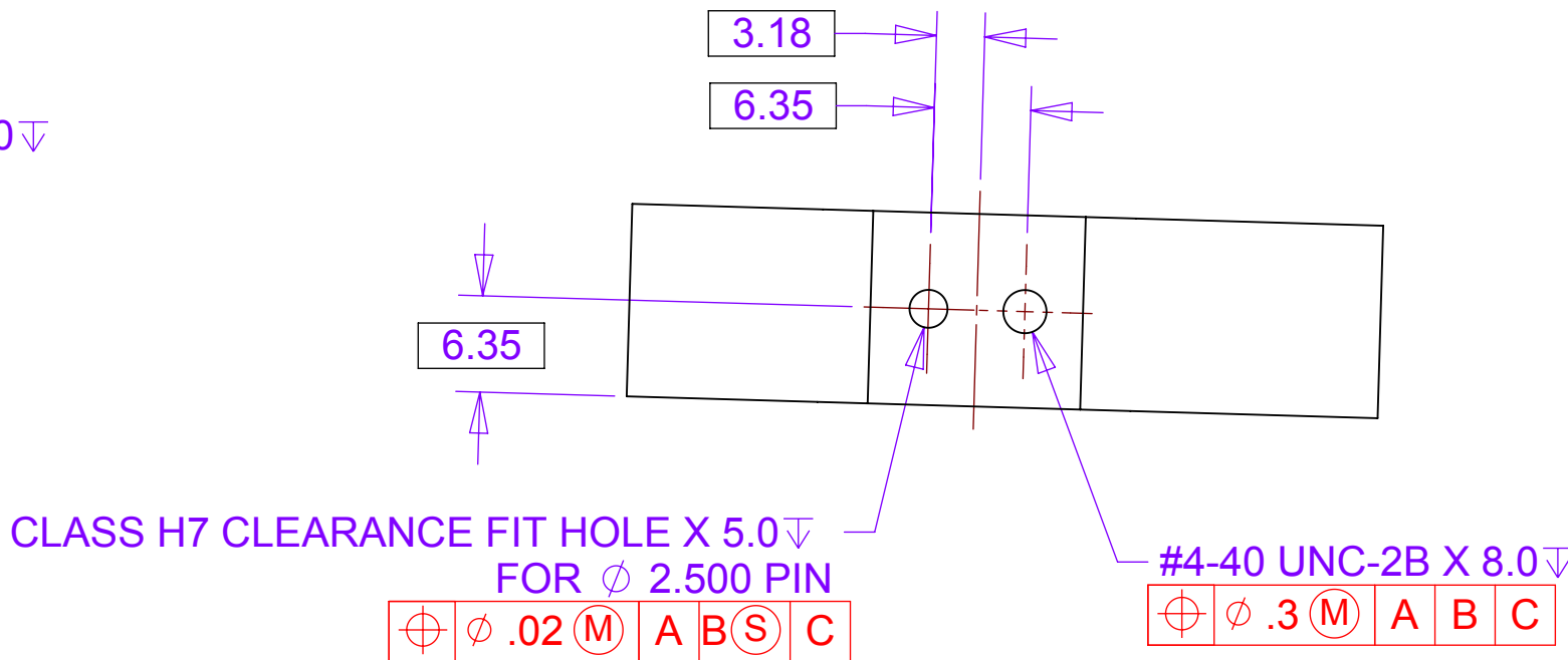
SECTION B-B
